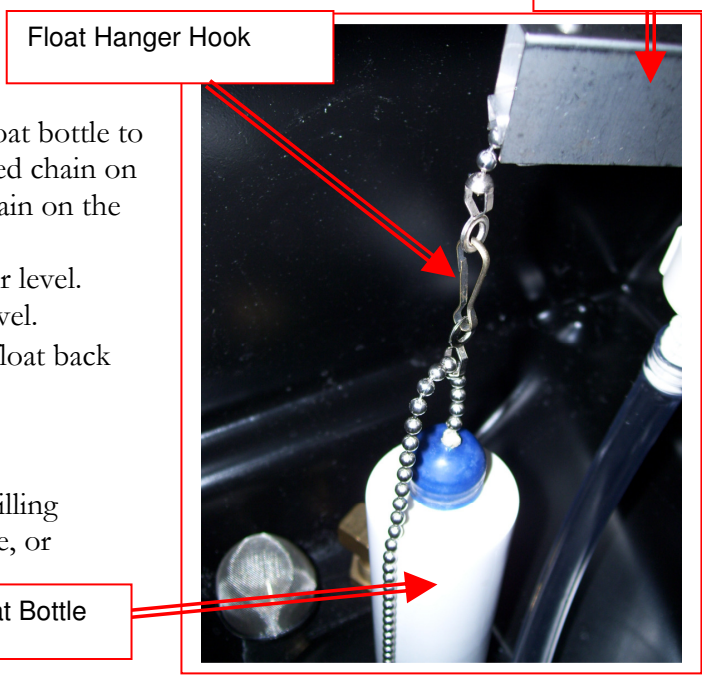
Float Valve
